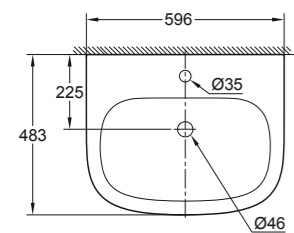
39 337 000 39 337 00H* Countertop basin 60 cm
