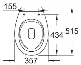
39 431 000 Floorstanding WC, wash down, vertical outlet
