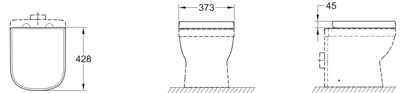
39 459 000 Seat & cover w/o soft close for compact toilet
