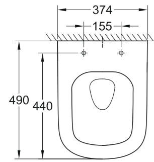
39 206 000 39 206 00H* Compact wall hung WC, wash down
