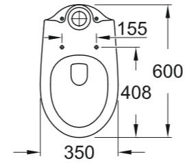
39 428 000 Floorstanding WC close coupled, wash down, horizontal outlet
