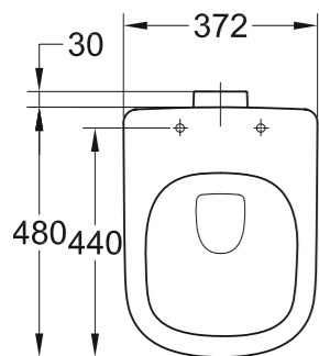
39 329 000 39 329 00H* Floorstanding WC, wash down, universal outlet
