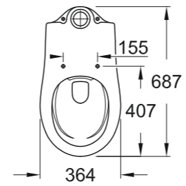
39 429 000 Floorstanding WC close coupled, wash down, vertical outlet
