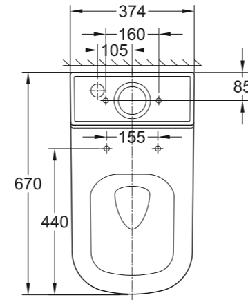
39 338 000 39 338 00H* Floorstanding WC, close coupled, wash down, universal
