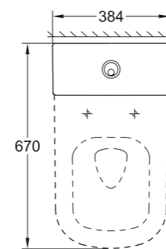
39 332 000 Cistern with bottom inlet
