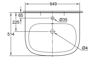
39 323 000 39 323 00H* Wall hung basin 65 cm
