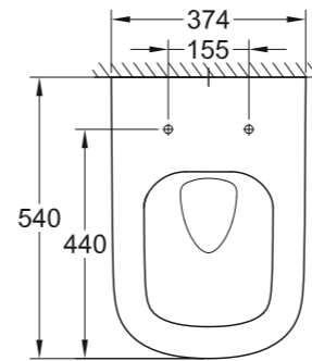
39 339 000 39 339 00H* Floorstanding WC, back to wall, wash down, universal outlet
