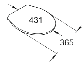
39 429 000 Floorstanding WC close coupled, wash down, vertical outlet
