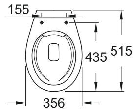
39 430 000 Floorstanding WC, wash down, horizontal outlet
