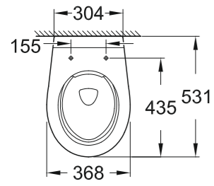
39 427 000 Wall hung WC, wash down
