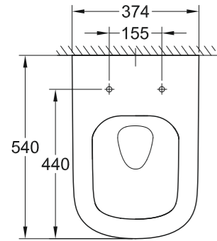
39 328 000 39 328 00H* Wall hung WC, wash down
