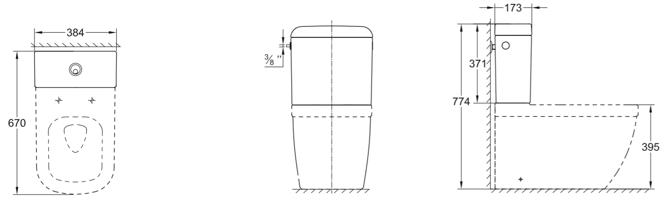
39 333 000 Cistern with side and back inlet outlet
